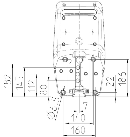
Abb. 7: Bohrmaße [mm]
